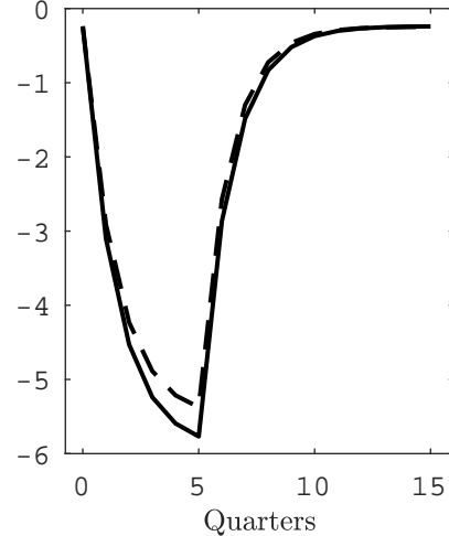
Average Inflation, \hat{\pi}_t
