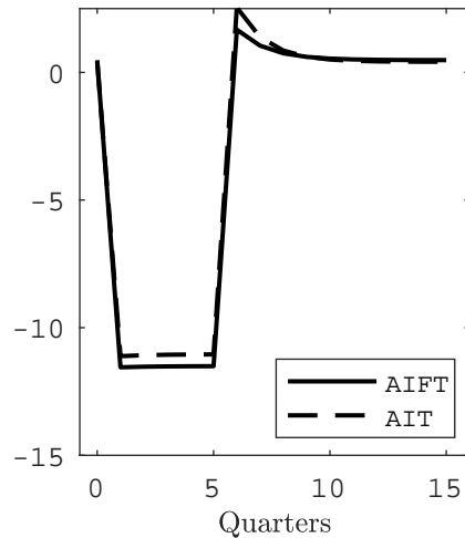
Output gap, y_t
